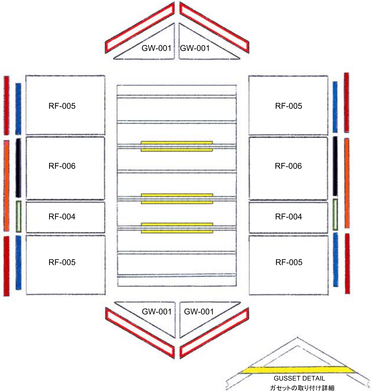
8X12(12x8) Shed
